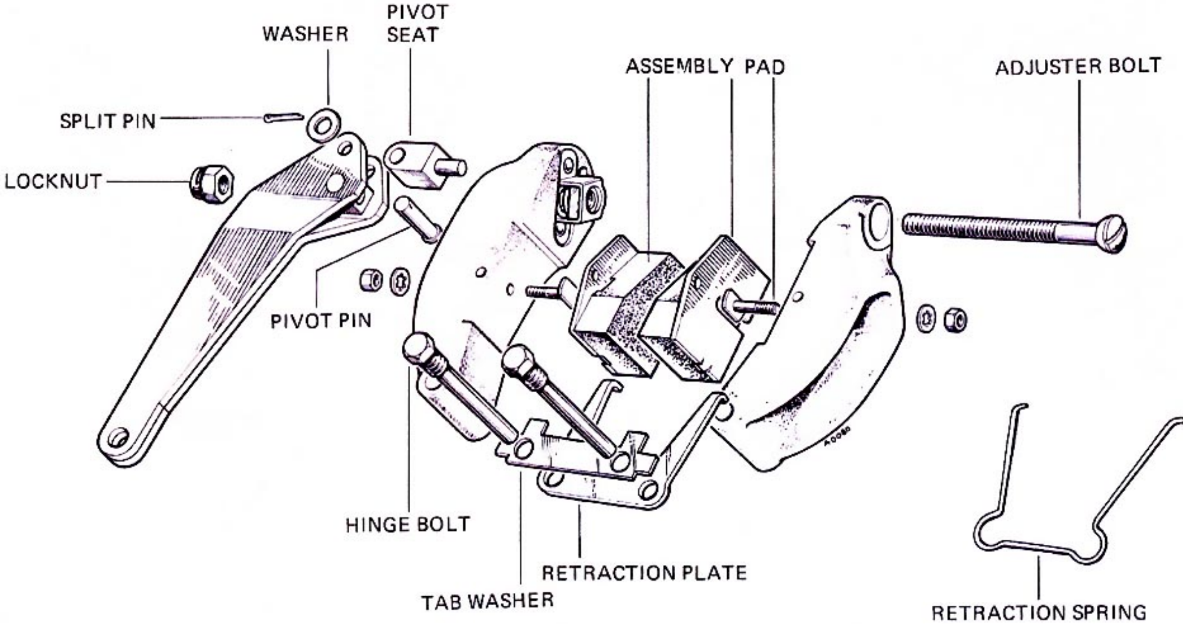
ILLUSTRATION NO. 5 MK I MANUALLY ADJUSTED HANDBRAKE
