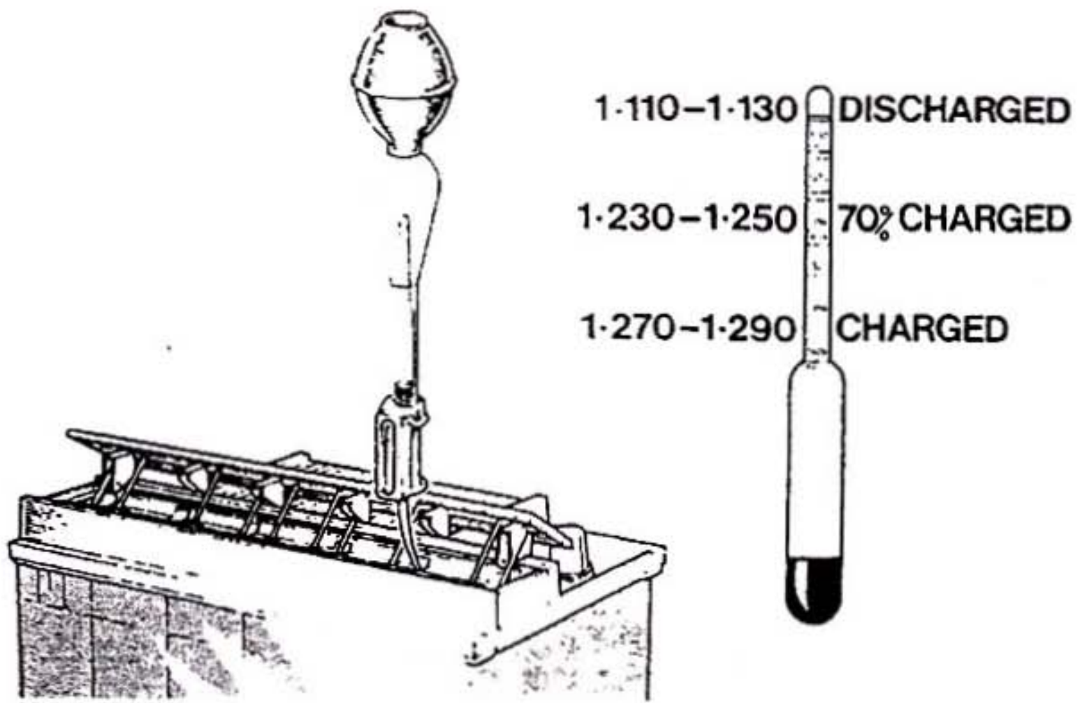
Fig. 7 Hydrometer test
