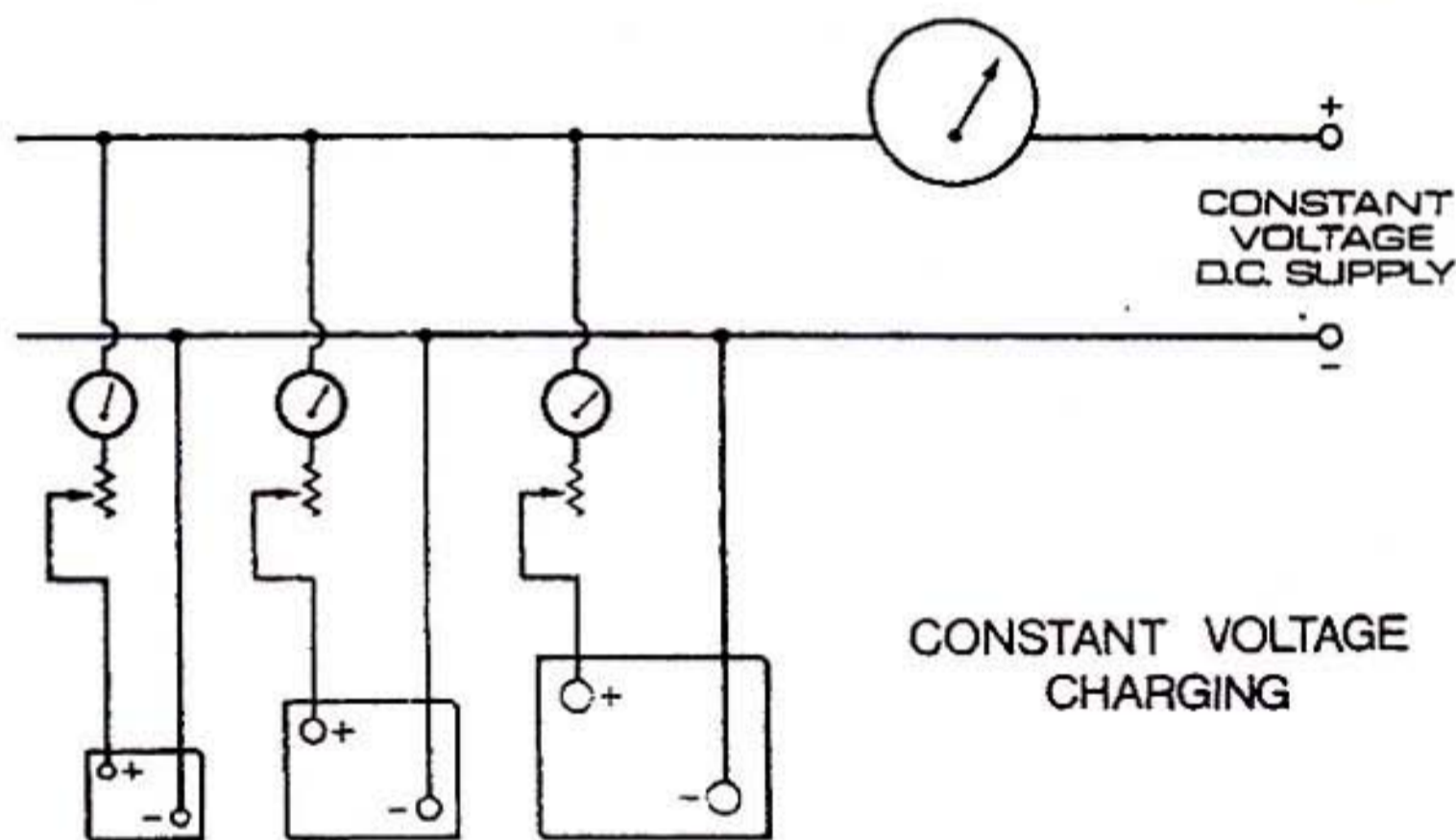
Fig. 6 Constant voltage charging
