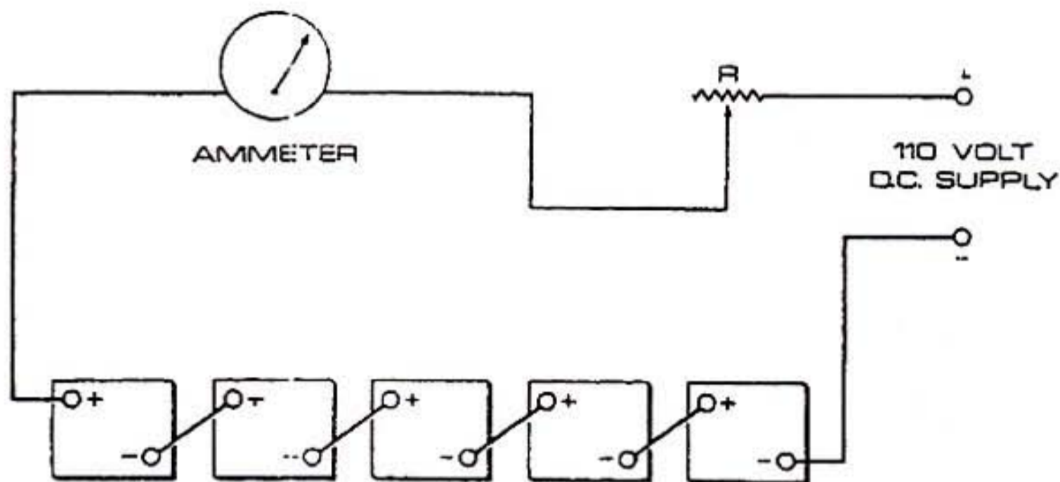
Fig. 5 Constant current charging
