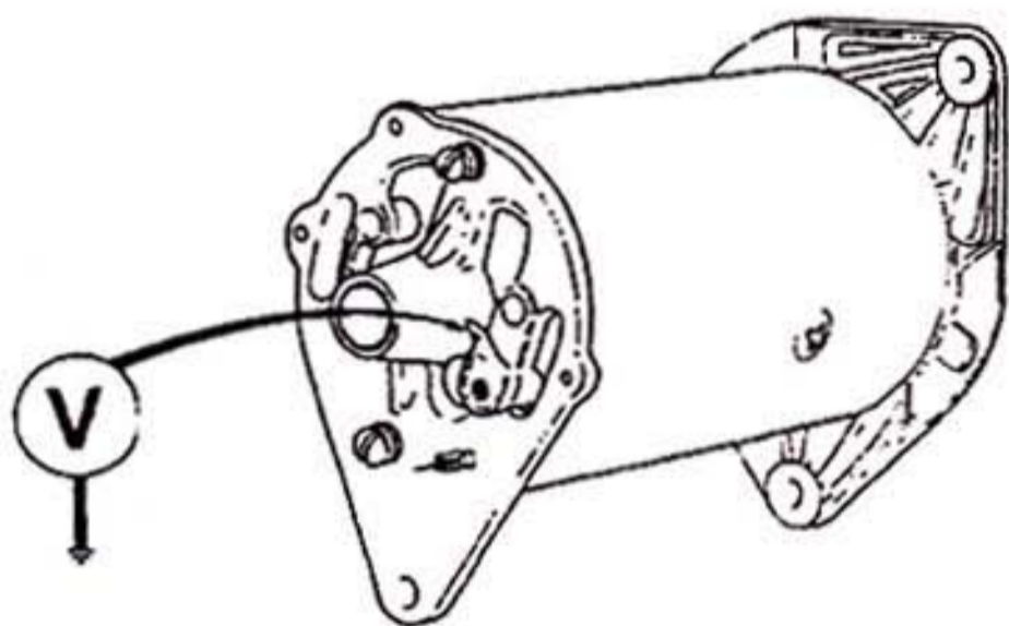
Fig. 57 Testing the armature circuit
