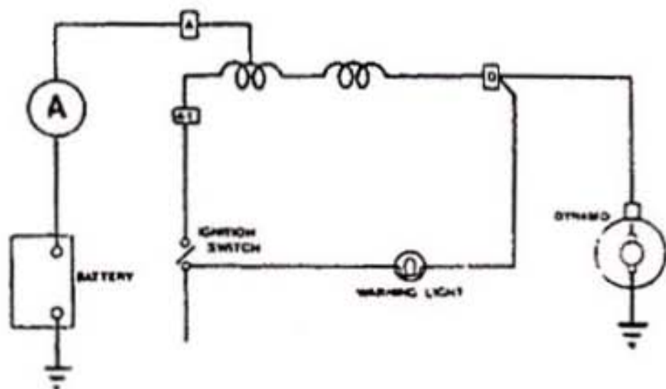
Fig. 63 Ignition warning light circuit
