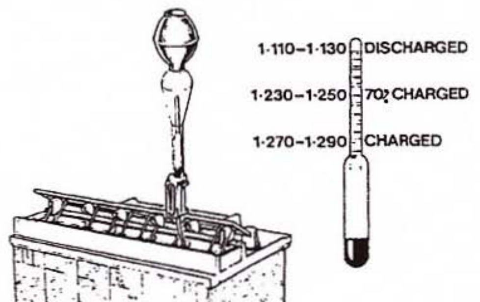
Fig. 55 Hydrometer test
