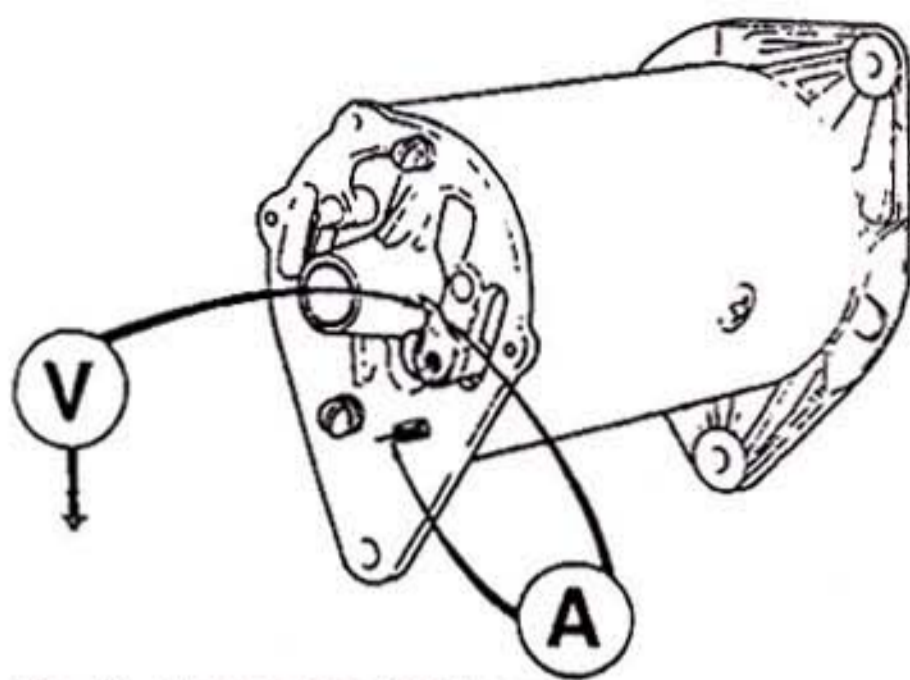
Fig. 58 Testing the field circuit
