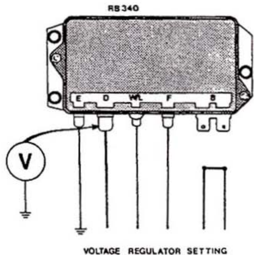
Fig. 64 Checking the voltage regulator setting
