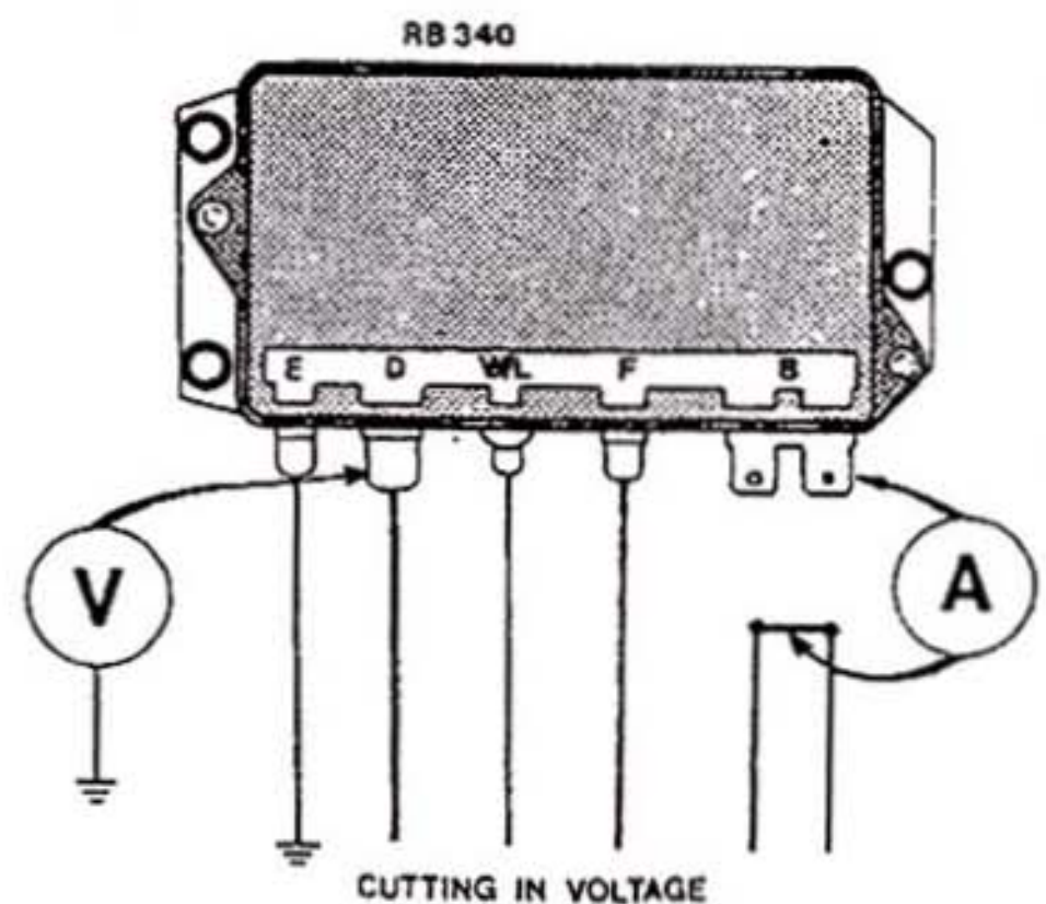
Fig. 65 Checking the cutting-in voltage
