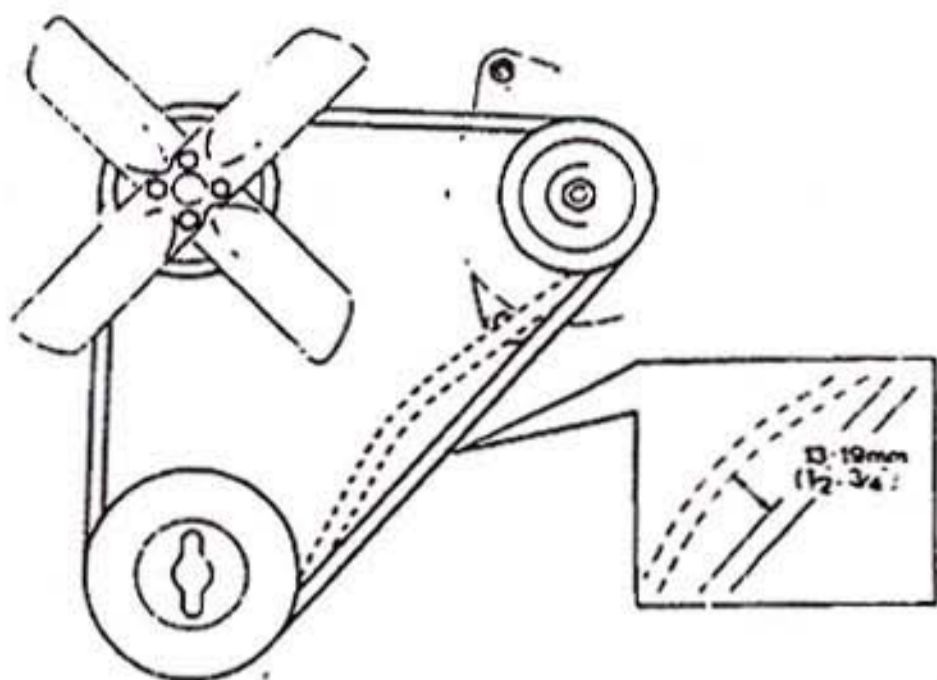
Fig. 56 Drive belt tension
